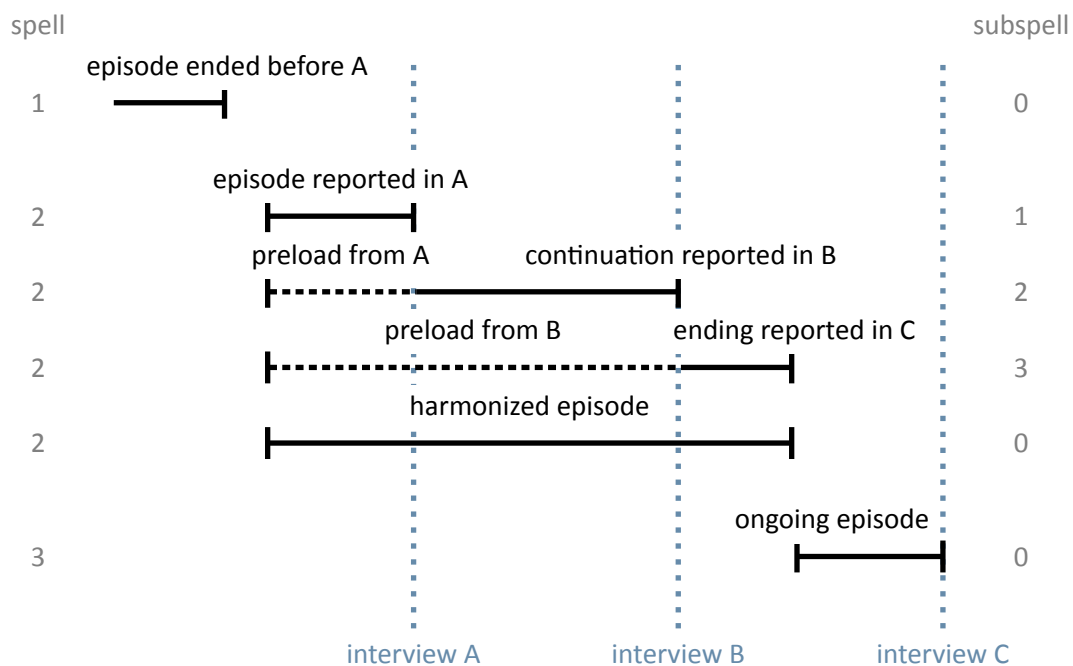
Figure 21: Logic of subsPELLs
