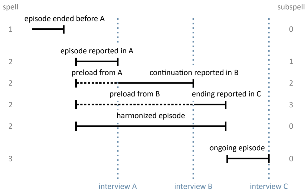
Figure 17: Logic of subsPELLs
